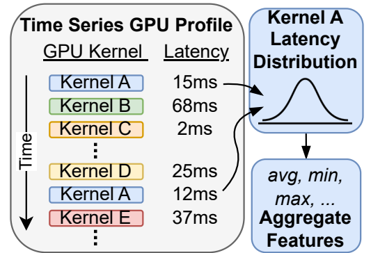
Fig. 2. Collection of aggregate GPU profiles without preserving the kernel execution order.
